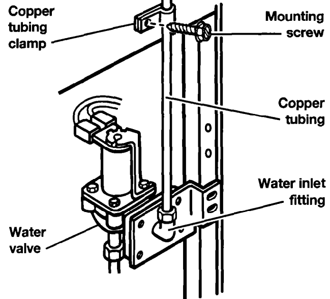
Style #2 valve
