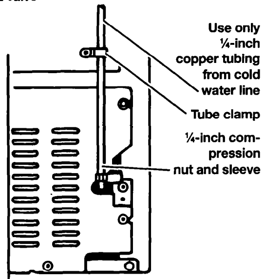
Style #2 valve
